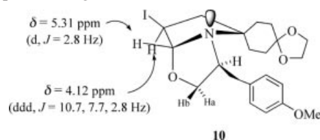
Figure 1. Assignment of the stereochemistry of 10 on the basis of coupling constants.
