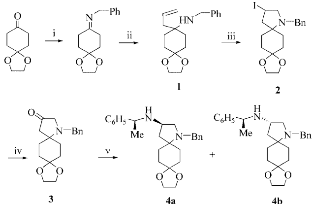
Scheme 2. Synthesis of enantiopure 3-amino-1-azaspiro[4.5]decan-8-ones: (i) \text{C}_6\text{H}_5\text{CH}_2\text{NH}_2 , 4 Å molecular sieves, \text{CH}_2\text{Cl}_2 , room temp., 5 h; (ii) \text{CH}_2=\text{CHCH}_2\text{MgBr} , \text{CH}_2\text{Cl}_2 , room temp., 95% for the two steps; (iii) \text{I}_2 , \text{NaHCO}_3 , \text{CH}_2\text{Cl}_2/\text{H}_2\text{O} , room temp., 12 h, 73%; (iv) \text{AgBF}_4 , DMSO, room temp., 12 h, quantitative; (v) ( S )-1-phenylethylamine, \text{NaCNBH}_3 , THF, room temp., 24 h, 72%.
